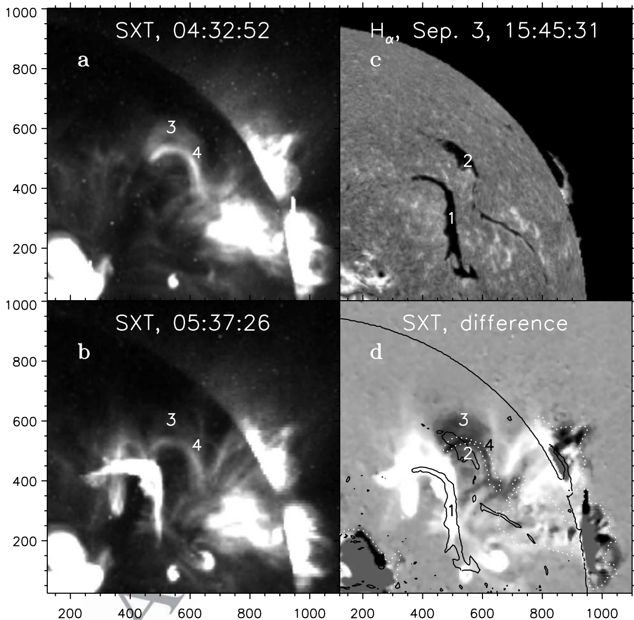
Figure 1. Soft X-ray and H \alpha images. (a) and (b) Preeruptive and posteruptive Yohkoh/SXT images (AlMg filter) and (d) their difference; (c) H \alpha filtergram, Big Bear Solar Observatory, 3 September 2000, 1546 UT (the previous day). Black contours in Figure 1d delineate filaments from the H \alpha image, and white dotted contours delineate bright loops in the preeruptive SXT image. Digits label filaments (1 and 2), broad dimming (3), loop structure (4).
