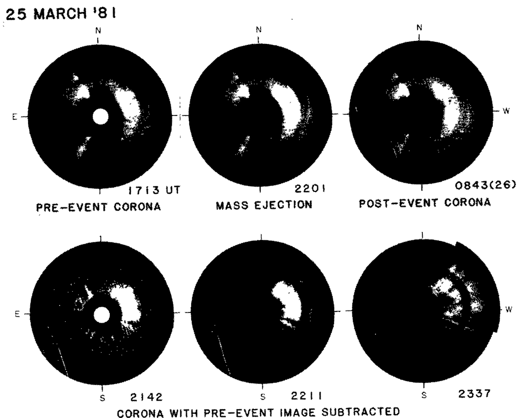
Figure 1 The CME of 25 March 1981, observed with the Solwind coronagraph. The top images are direct images, but the bottom images are difference images formed by subtracting a base image from the CME image. The solid white circles in the images on the left side indicate the solar disk. From N. R. Sheeley, Jr.
