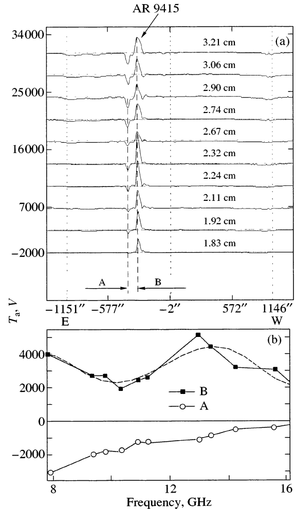
Fig. 4. (a) Polarization scans for the Sun (in antenna temperatures) on April 8, 2001, 9 h 15 m UT. AR 9415 lies in the eastern part of the solar disk and has a bipolar polarization pattern in the from of sources A and B. Source B exhibits a rise in intensity at short wavelengths, while source A shows no such dependence. (b) The spectra of the western (B) and eastern (A) sources in AR 9415. Source A shows a monotonic rise in left-hand circular polarization; source B of left-hand polarization exhibits a rise of the spectrum at short wavelengths. The dotted line represents a power-law polynomial fit.
