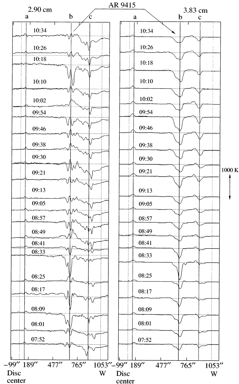
Fig. 8. An example of the dynamic polarization behavior for the FPAR 9415 at two wavelengths inside and outside the mode coupling region. The observations were carried out from 7 h 52 m until 10 h 34 m UT with an 8-min interval between the scans.
