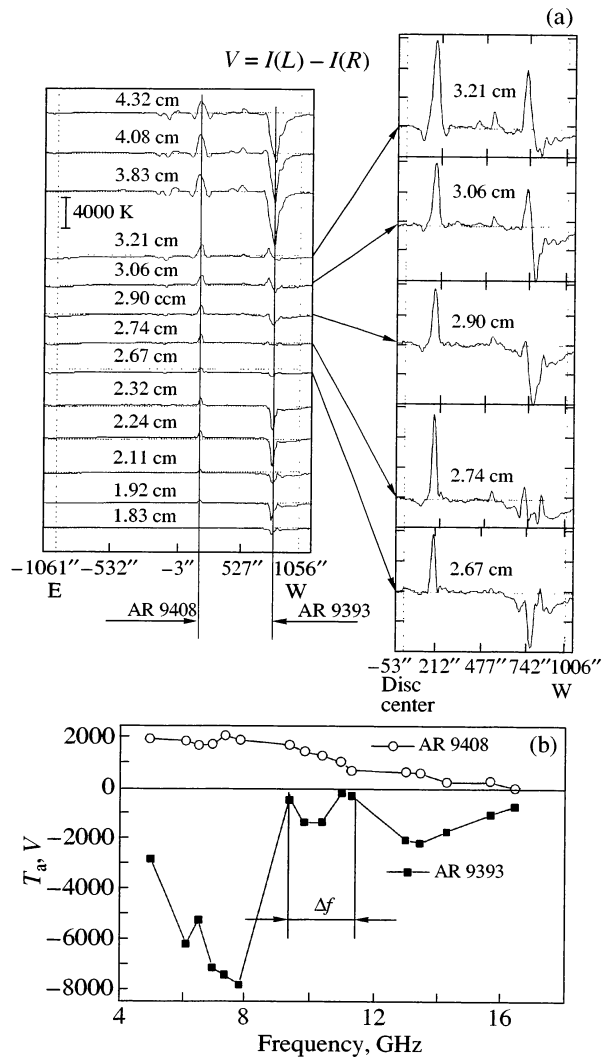
Fig. 5. (a) Polarization scans for the Sun on April 1, 2001, 9 h 17 m UT. AR 9393 lies in the western part of the solar disk and has a simple polarization pattern at short (2.32 cm or shorter) and long (3.83 cm or longer) wavelengths. The scans in the wavelength range from 2.67 to 3.21 cm are shown on the right on a large scale. This range exhibits a complex pattern of mode coupling with the appearance of narrow pointlike sources, with sharp spectral slopes, polarization inversions, and a low degree of polarization. (b) The circular polarization spectra for the stable AR 9408 and FPAR 9393. Here, \Delta f is the width of the frequency band in which abrupt variations occur at a low level of the polarized signal.
