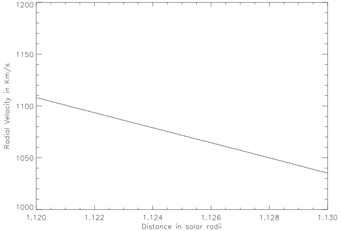
Figure 3.9 Fiber source radial velocity vs. distance in solar radii.
