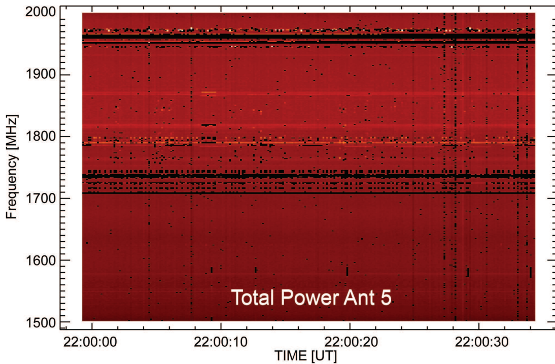
Figure 4.4 The RFI-cleaned dynamic spectrum obtained from the same data displayed in Figure 4.1, but with frequency resolution reduced by a factor of 8 in order to improve the SK statistics ( M = 1952 contiguous PSD estimates). To allow a better comparison with Figs. 4.1 and 4.2, no subchannel integration has been performed.
