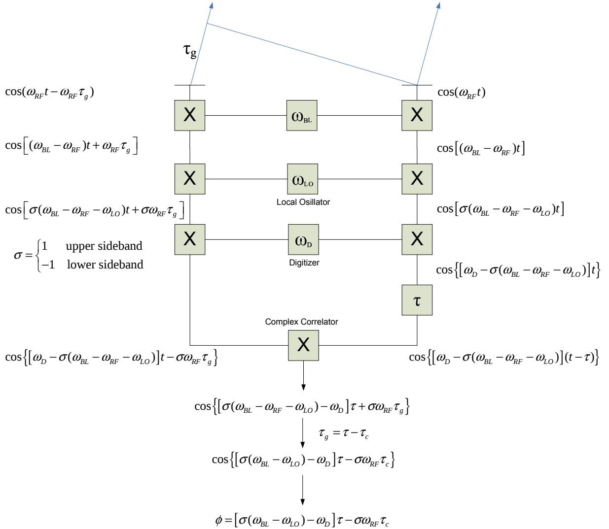
Figure 2.12 Origin of the phase correction needed due to two stages of explicit downconversion and one stage of implicit downconversion due to digitizer.
