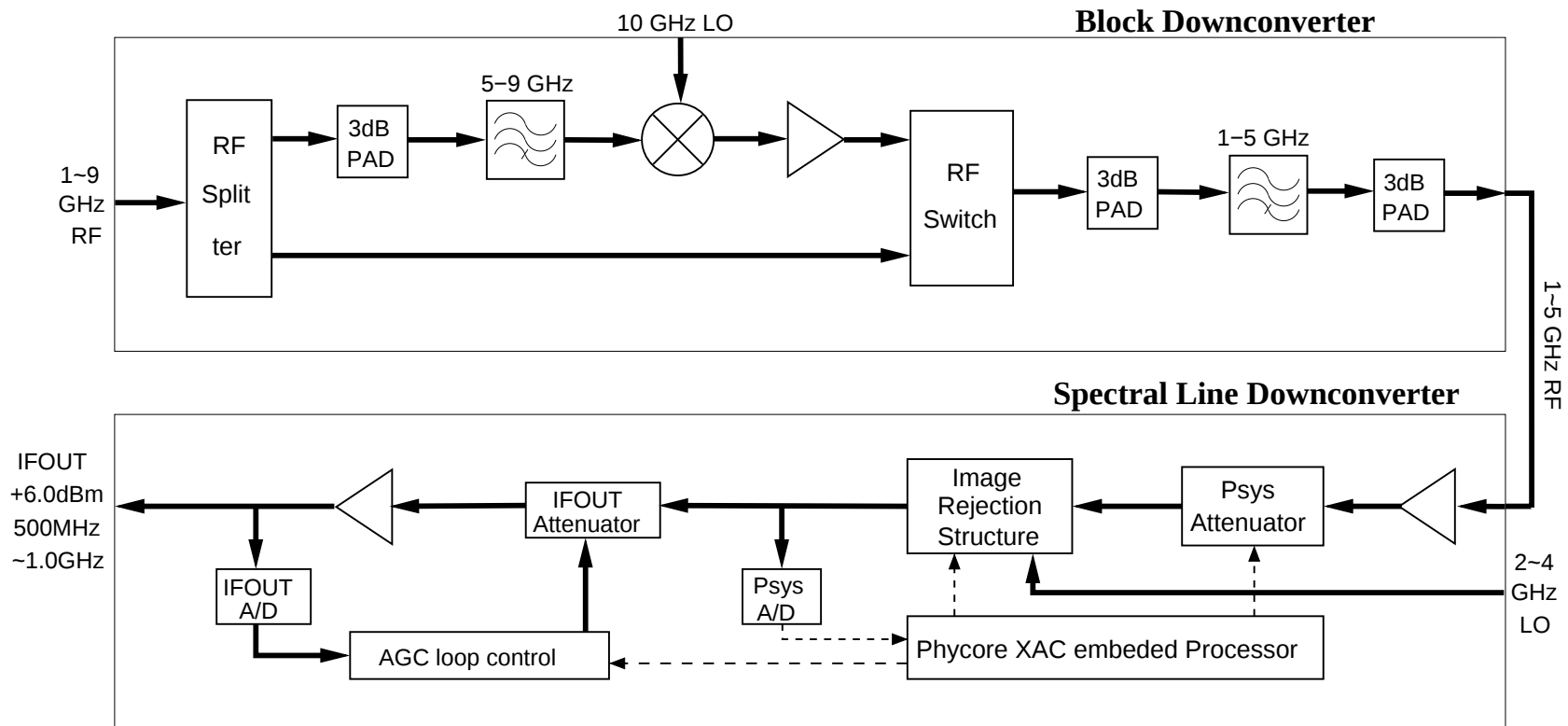
Figure 2.4 The two stages of downconversion: block downconverter (upper panel) and spectral-line downconverter (lower panel). The digitizer performs an implicit third stage of downconversion due to its sampling below the Nyquist frequency.
