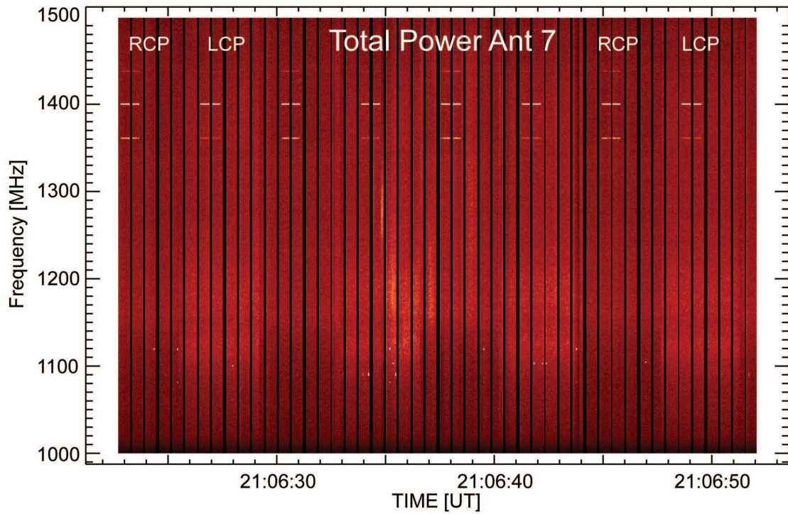
Figure 4.5 Total power dynamic spectrum of a weak solar radio burst recorded on 2006 April 05, around 21:06:30 UT, in the 1-1.5 GHz frequency band. The time resolution of the dynamic spectrum is 25 ms and the frequency resolution is 1 MHz. The vertical black stripes in the plot represent variable time gaps needed to dump each separate acquisition on the storage media. Four on/off periodic RFI signals can be seen at 1190, 1360, 1400, and 1440 MHz, as well as a few narrowband features scattered below 1200 MHz, most likely due to aircraft distance measuring equipment. RCP and LCP labels indicate a few of the periodic changes in the background intensity, every about 4 s, due to periodic switching of the observed circular polarization, which is the default mode of operation of OVSA.
