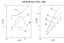
Figure 1: Flux density and brightness temperature spectra of AR 8108 details. Details A and B identified with spots have spectra characteristic of cyclotron radiation with some addition of bremsstrahlung in the case of B. The spectrum of detail H is nonthermal, typical of halo. Detail X, identified with streamer, has a flat flux spectrum characteristic of thermal bremsstrahlung.
